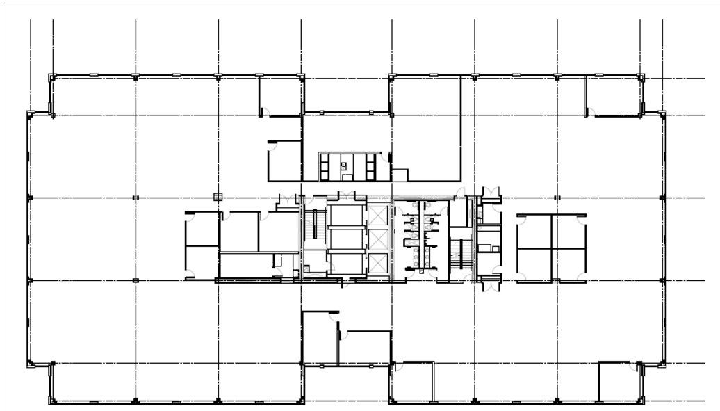
Typical Floor Plan—26,000 SF
